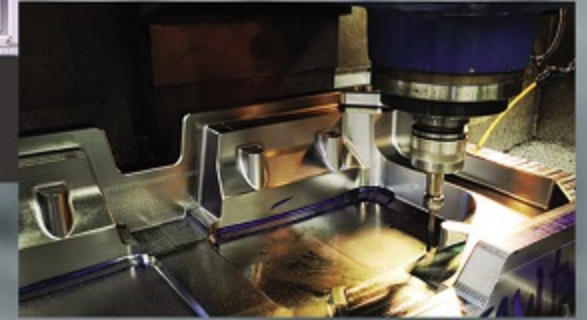
Mold Making
